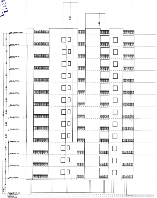
REAR SIDE ELEVATION
